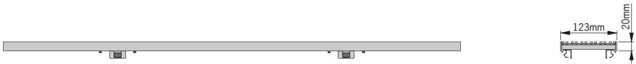
Side elevation
