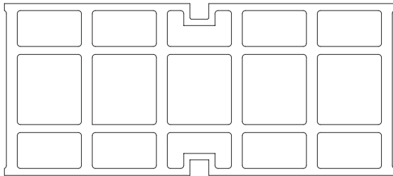
Shoring of the grate of nominal width 200 (500 x 223 mm)
